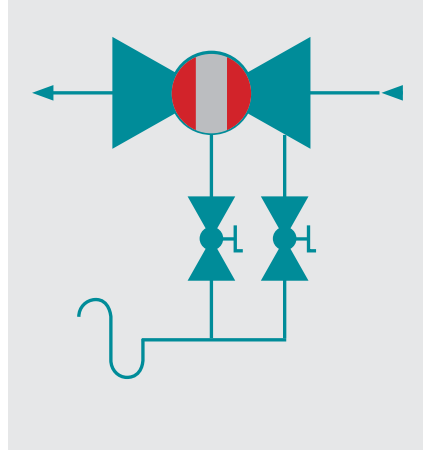
Type DBI-B&I
